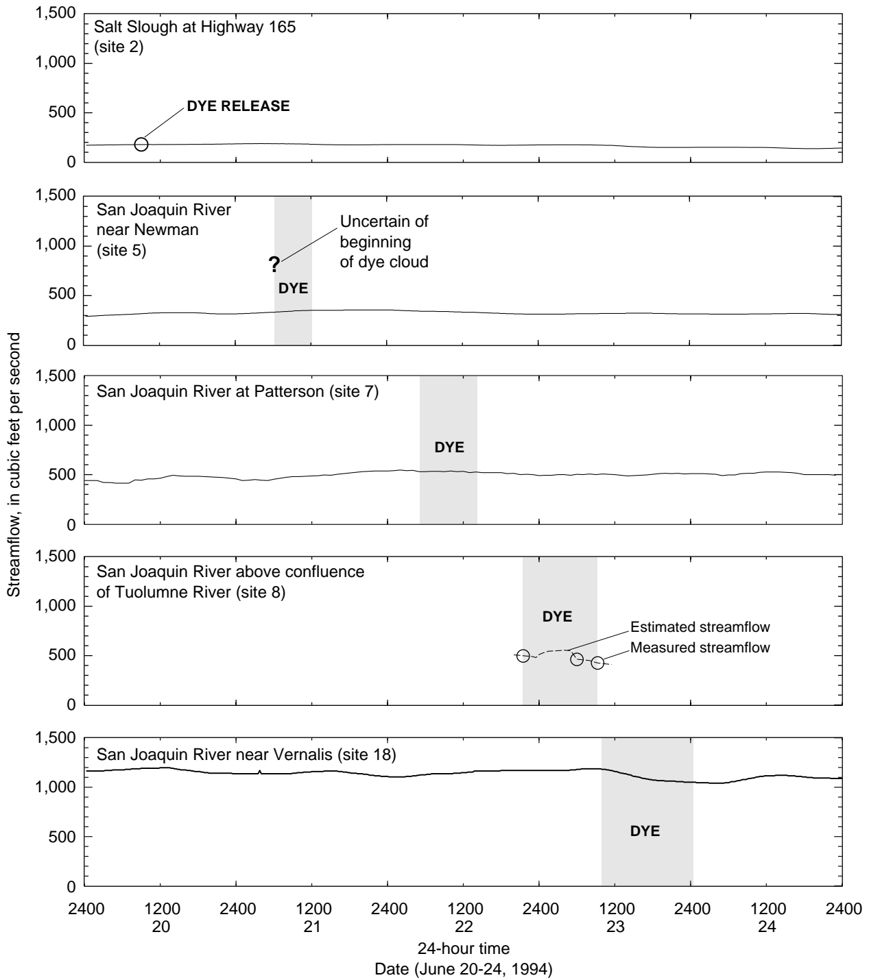
Figure 4. Presence of dye cloud relative to streamflow at dye release site and at sampling sites with streamflow data for the June 1994 study (site numbers refer to figure 1).
