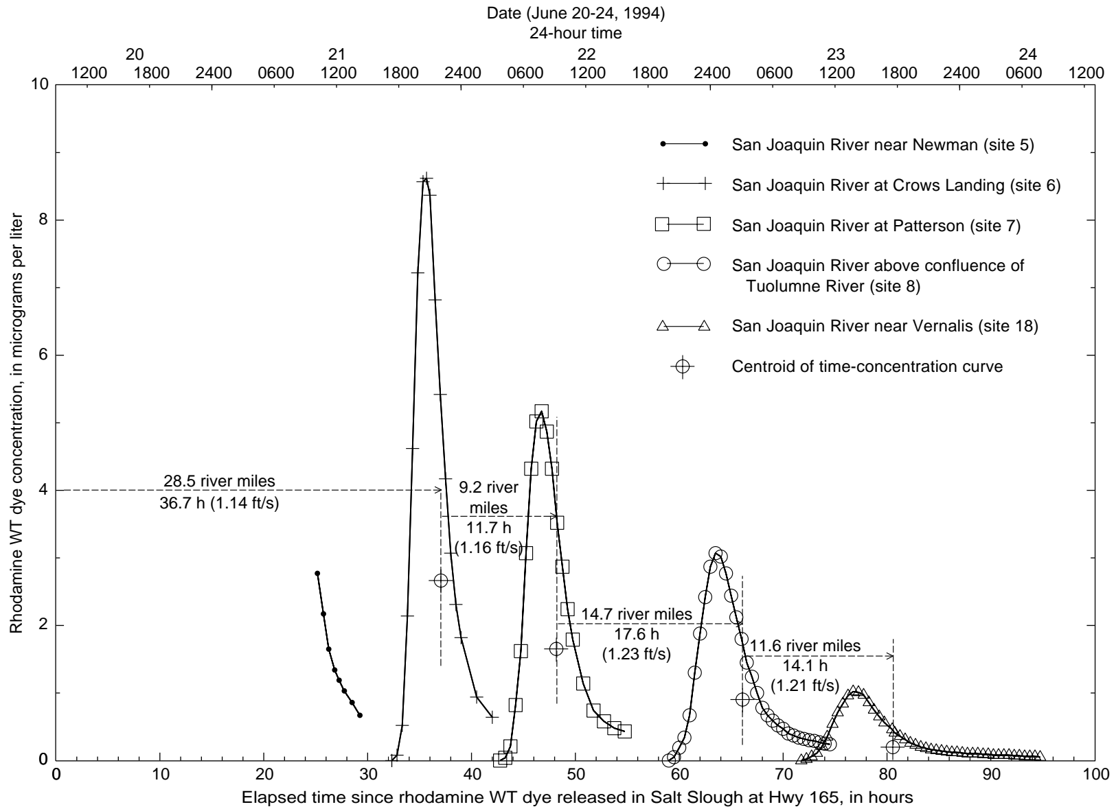
Figure 5. Time-concentration curves at sampling sites for June 1994 study. Dye traveltimes and average velocities (shown below horizontal dashed lines labeled with river miles) are based on centroid of time-concentration curves (site numbers refer to figure 1). ft/s, foot per second; h, hour.
