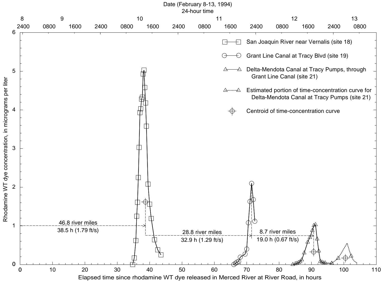
Figure 3. Time-concentration curves at sampling sites for February 1994 study. Dye travel times and average velocities (shown below horizontal dashed lines labeled with river miles) are based on centroid of time-concentration curves at sites 18 and 21; based on peak concentration at site 19 (site numbers refer to figure 1). ft/s, foot per second; h, hour.
