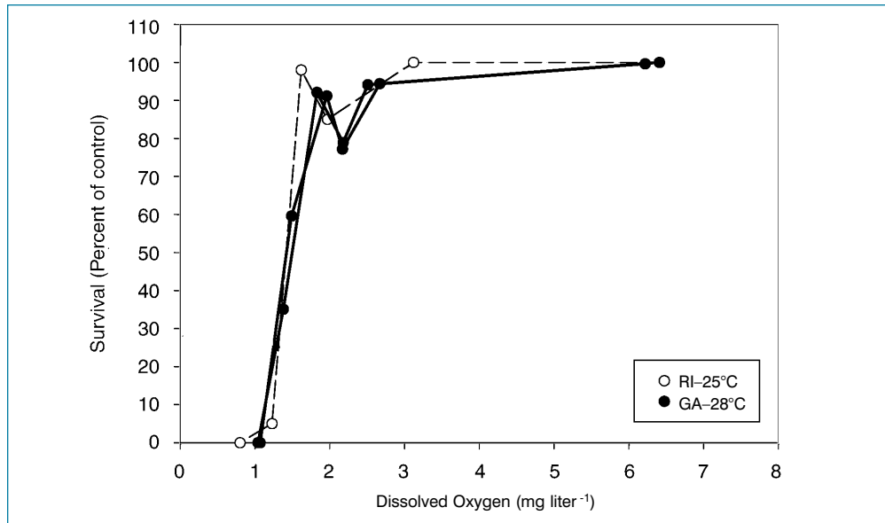
Figure B-5. Ninety-six hour dose-response for larvae of the inland silverside Menidia beryllina exposed to various levels of low dissolved oxygen at two temperatures. Open circles are for a test conducted with a population from Rhode Island (RI) (25°C) and closed circles are for two tests with a population from Georgia (GA) conducted at 28°C. The Rhode Island data are from a test listed in Poucher and Coiro (1997). Tests were initiated with 7-day-old larvae.
