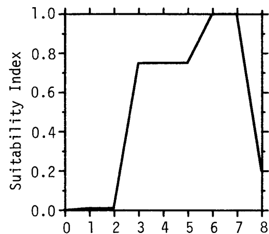
Figure 5. SI curves for rainbow trout adult velocity, depth, substrate, and temperature.
