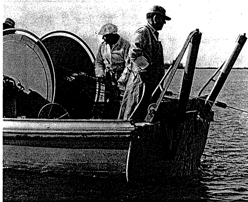
FIGURE 14. Trammel net being wound onto powered net reel on the M.V. Striper , San Joaquin River at Prisoners Point; fall, 1965. Photograph by Richard J. Hallock.
