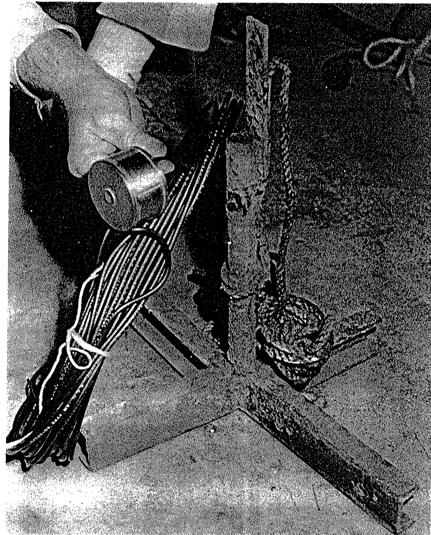
FIGURE 11. Hydrophone, iron stand used to hold it above the river bottom and lead-in cable. Photograph by Wm. F. Van Woert.
