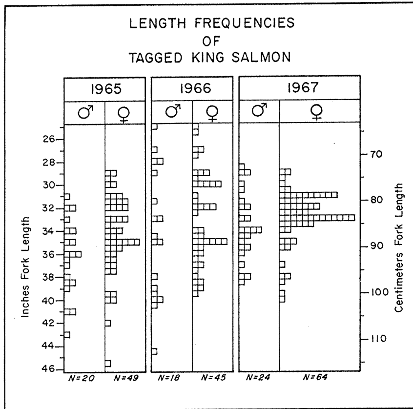
FIGURE 21. Length frequencies of tagged king salmon.
